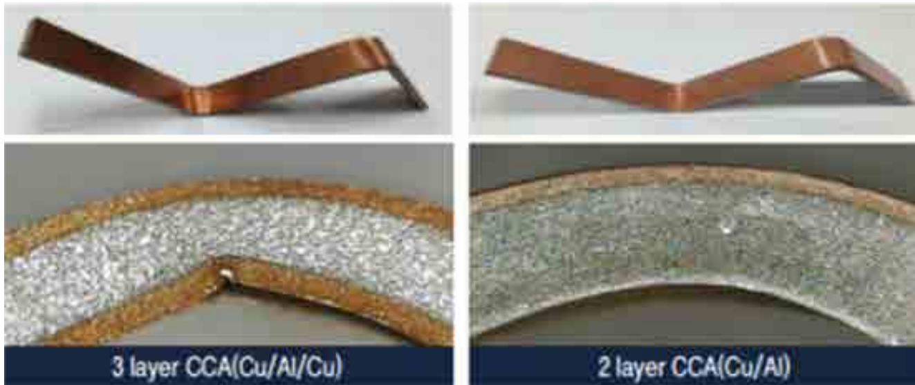
CCA Busbar
