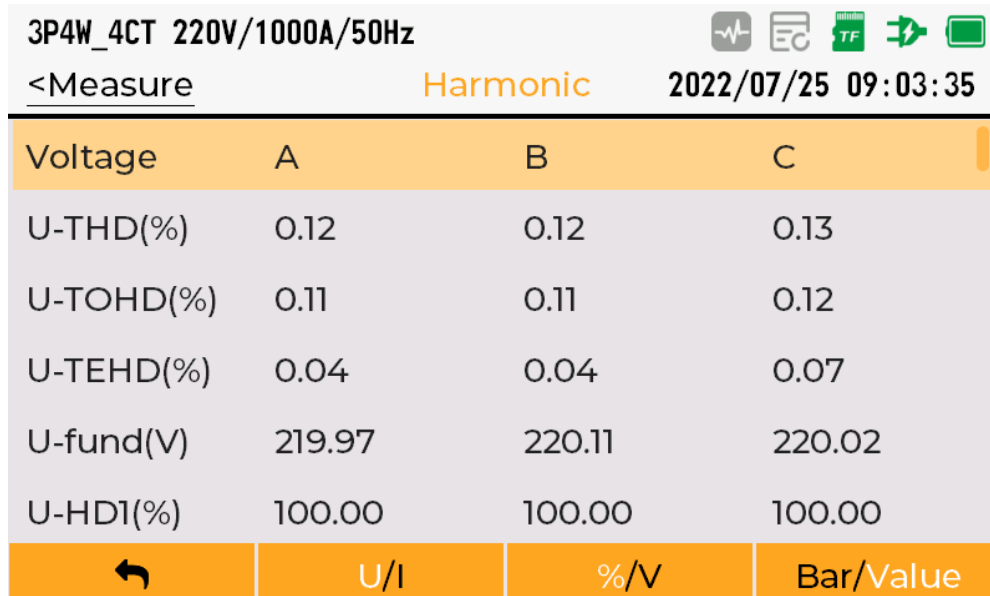
Figure 5-36 Harmonic value display
