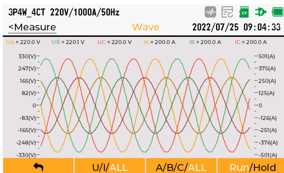
Figure 5-37 Voltage and current waveform display
