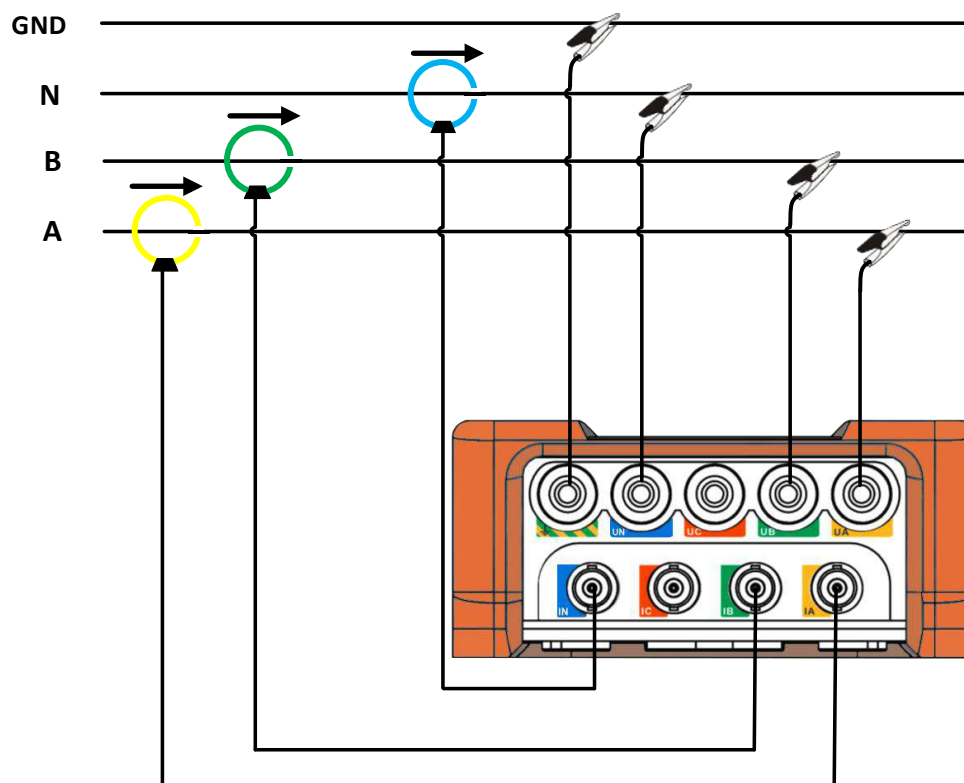
Figure 3-5 1P3W
