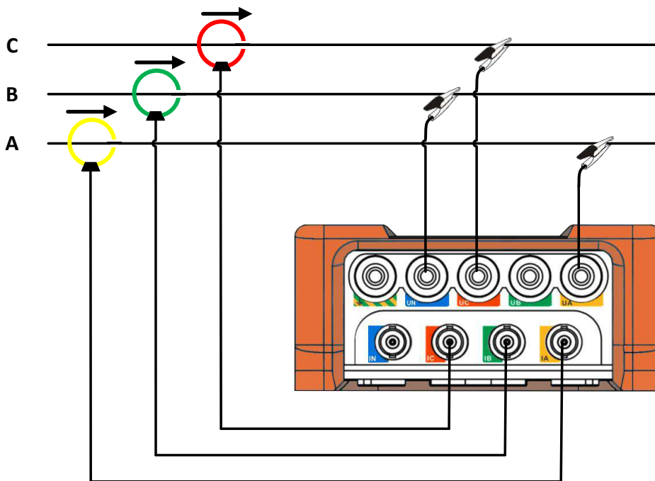
Figure 3-3 3P3W_3CT
