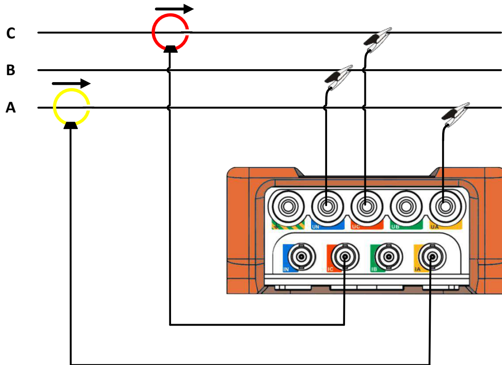
Figure 3-4 3P3W_2CT
