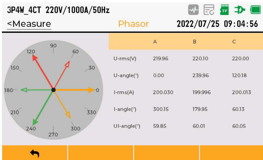
Figure 5-39 Vector diagram display
