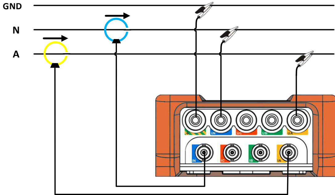
Figure 3-6 1P2W
