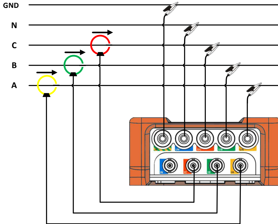
Figure 3-2 3P4W_3CT
