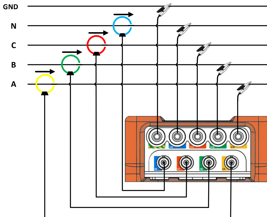
Figure 3-1 3P4W_4CT
